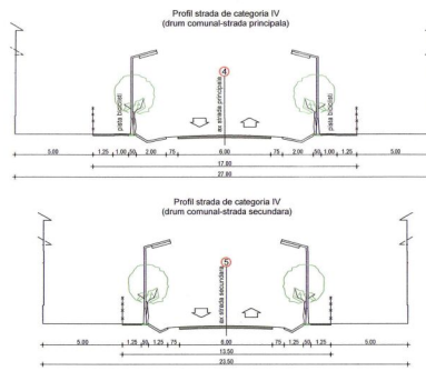
PROFILE CARACTERISTICE DE STRAZI scara 1/200
